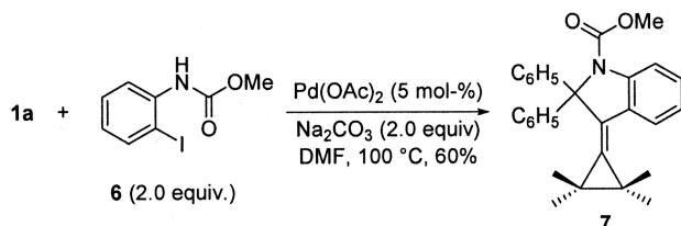
Scheme 1. \text{Pd}(\text{OAc})_2 -catalyzed coupling reaction of 1 with 6 .
